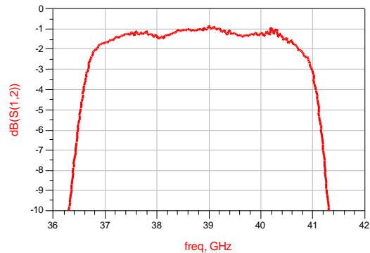
Passband loss VS frequency (T A =25°C)
