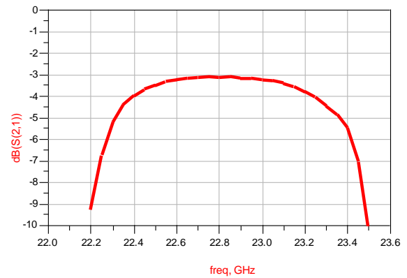
Passband loss VS frequency ( T_A=25^\circ\text{C} )
