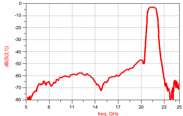
Distal inhibition vs frequency (T A =25°C)
