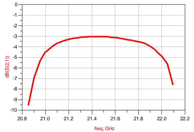
Passband loss vs frequency (T A =25°C)
